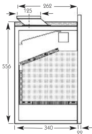
Inset Stove dimensions
